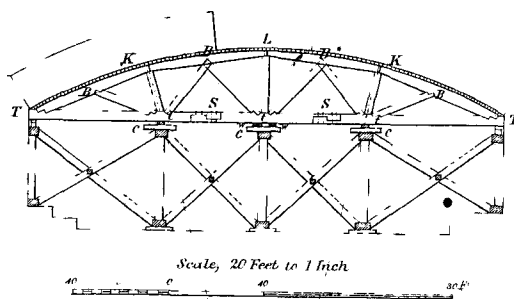
Fig. 1 End Elevation of Centre.
