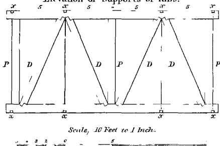
Fig. 3 Elevation of Supports of Ribs.
