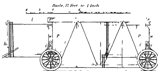
Fig. 3 Elevation of Supports of Ribs.
