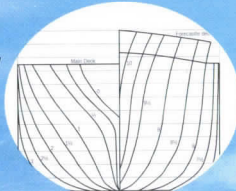
Ship Design
